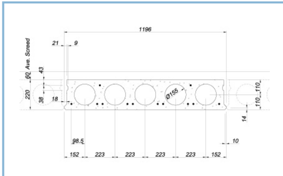
220 Thick 5 Core HC Slab
