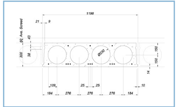
300 Thick 4 Core HC Slab
