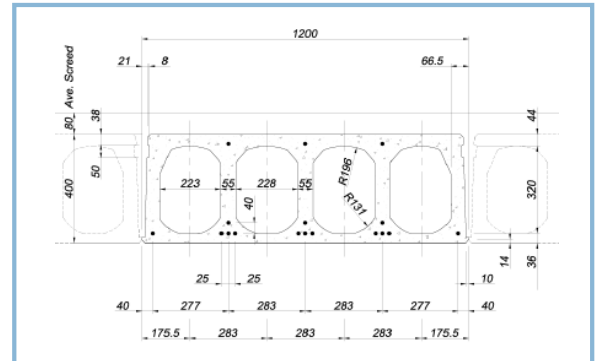
400 Thick 4 Core HC Slab
