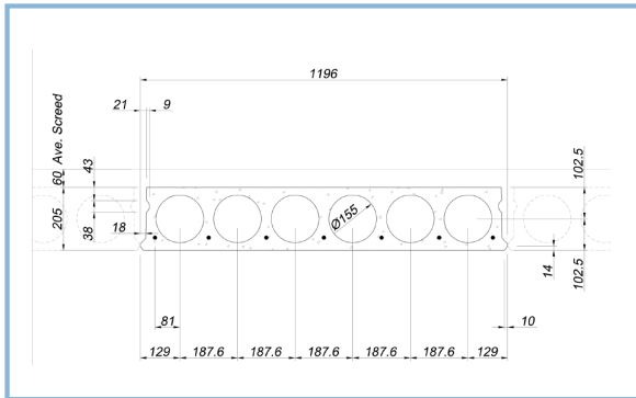
205 Thick 6 Core HC Slab
